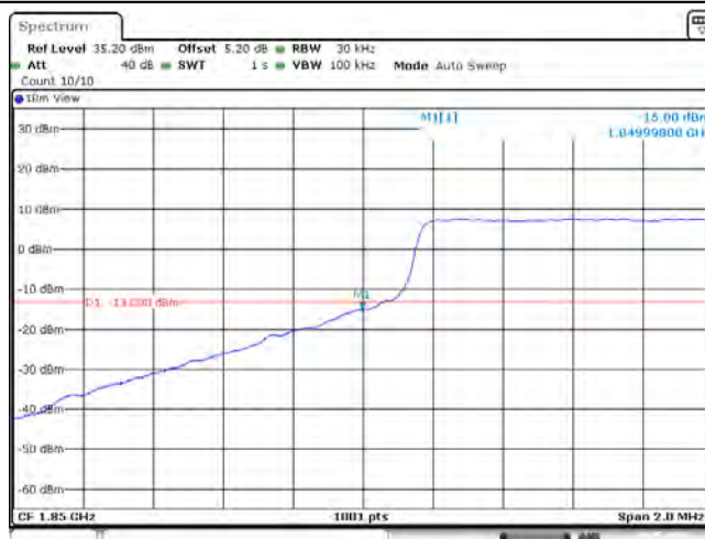
Band25_1.4MHz_16QAM_26047_6RB#0
