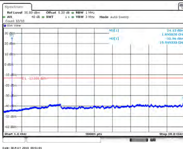
Band25_20MHz_16QAM_26140_1RB#0
