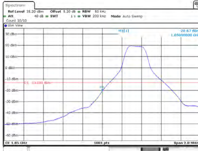
Band25_5MHz_QPSK_26065_25RB#0
