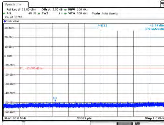
Band25_20MHz_16QAM_26140_1RB#0
