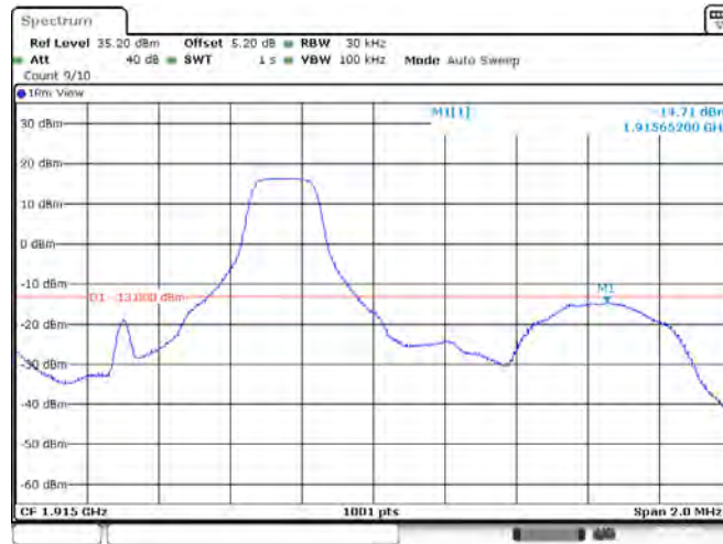
Band25_1.4MHz_QPSK_26683_6RB#0
