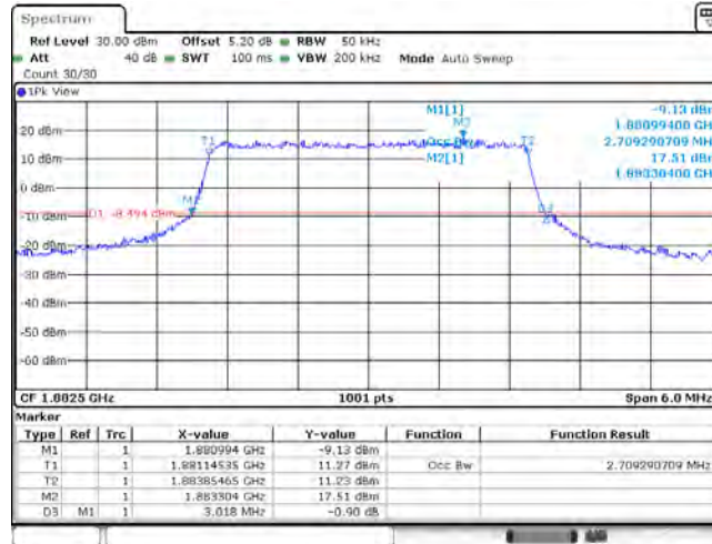
Band25_3MHz_QPSK_26365_15RB#0
