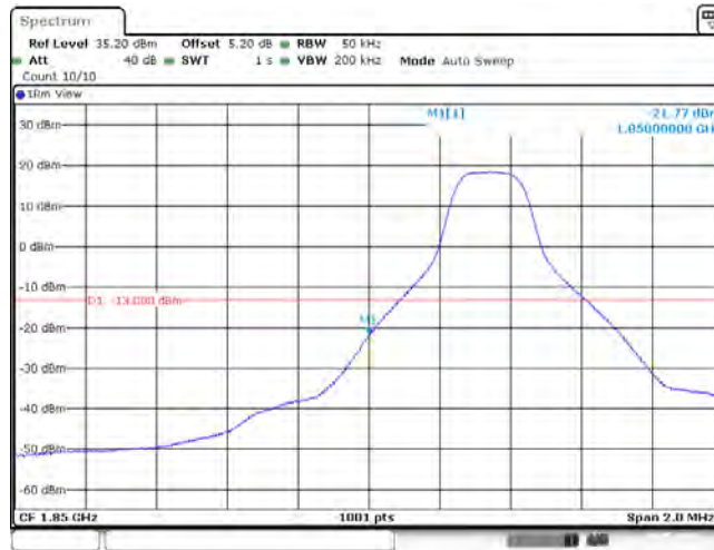
Band25_5MHz_16QAM_26065_25RB#0
