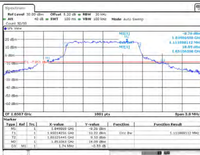
Band25_1.4MHz_QPSK_26047_6RB#0
