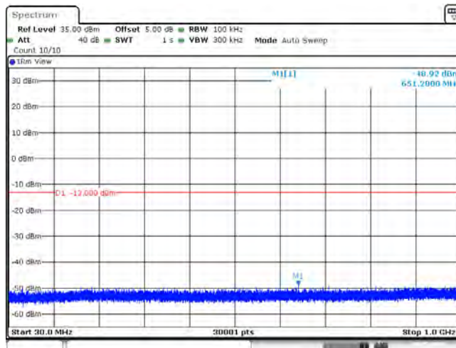
Band25_20MHz_16QAM_26365_1RB#0
