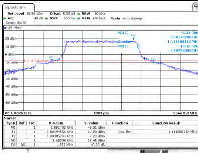
Band25_1.4MHz_QPSK_26365_6RB#0
