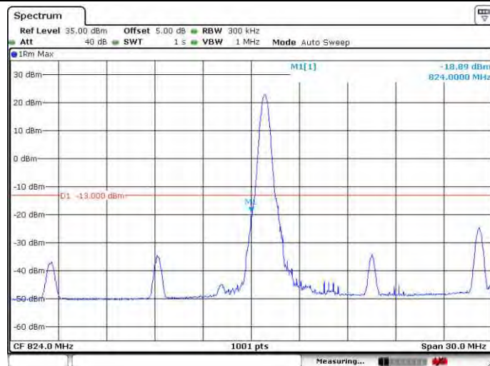
BAND 26_15MHz_16QAM_26865_75RB#0
