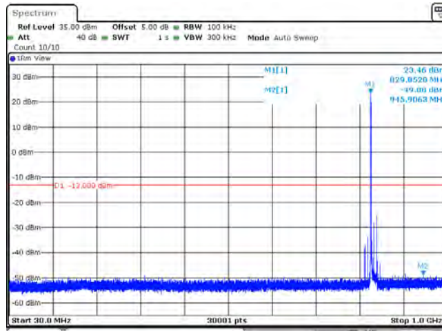
Band26_15MHz_QPSK_26915_1RB#0
