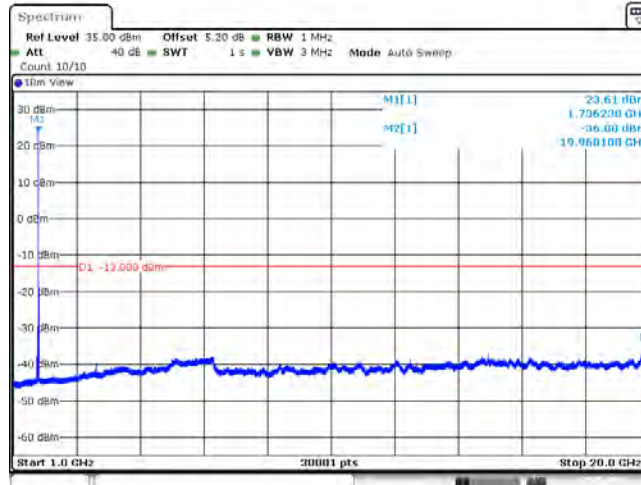
Band4_20MHz_QPSK_20300_1RB#0
