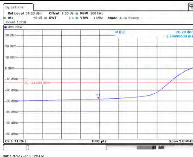
Band4_20MHz_16QAM_20300_1RB#99
