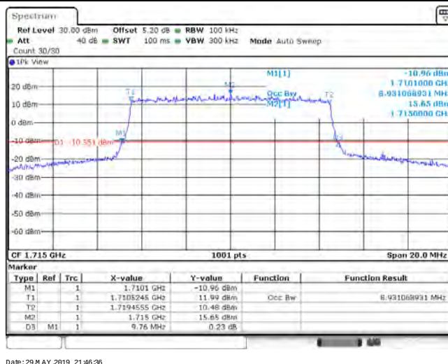
Band4_10MHz_QPSK_20175_50RB#0
