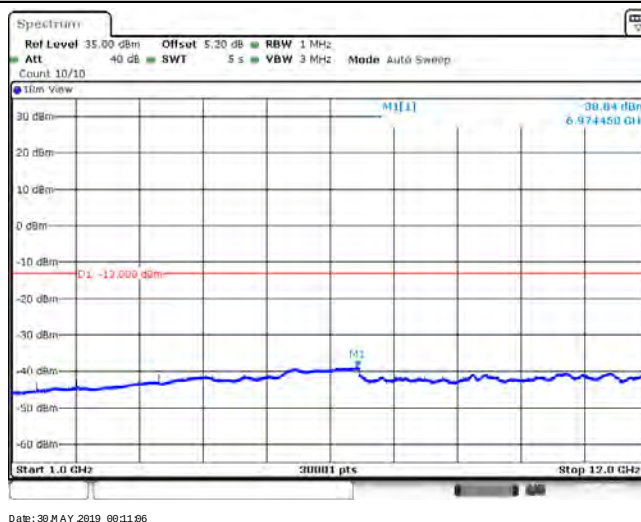
Band12_10MHz_16QAM_23130_1RB#0
