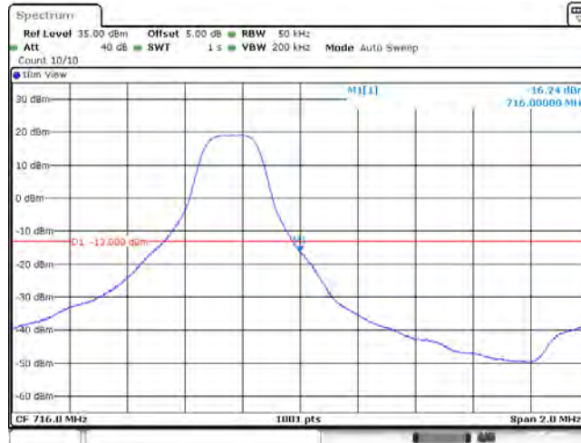
Band12_3MHz_QPSK_23165_15RB#0
