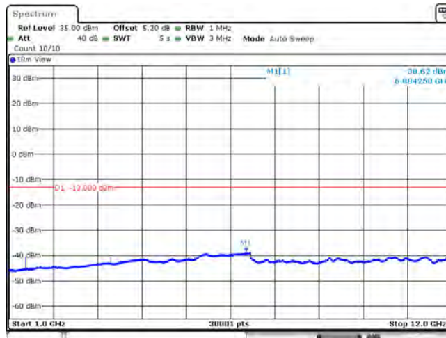
Band12_10MHz_16QAM_23095_1RB#0
