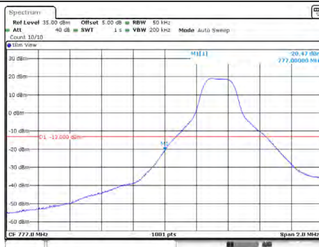
Band13_5MHz_QPSK_23205_1RB#0
