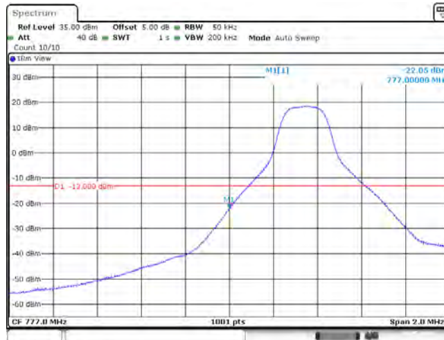
Band13_5MHz_16QAM_23205_25RB#0
