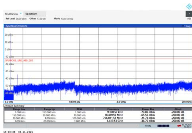
LTE Band 12 10MHz CH-High 9kHz~20GHz
