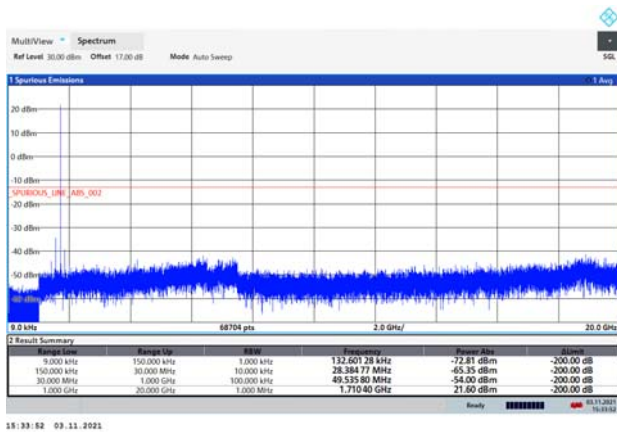
LTE Band 4 10MHz CH-Middle 9kHz~20GHz
