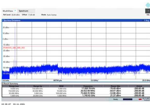
LTE Band 4 10MHz CH-High 9kHz~20GHz
