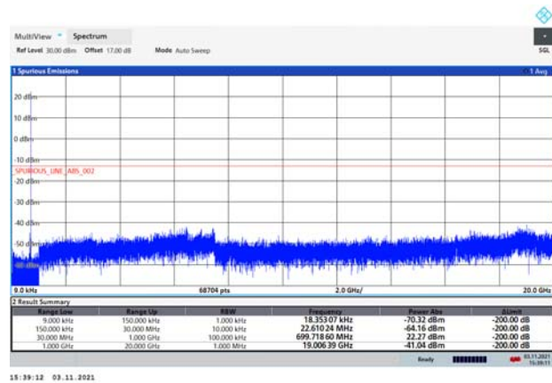
LTE Band 12 10MHz CH-Middle 9kHz~20GHz
