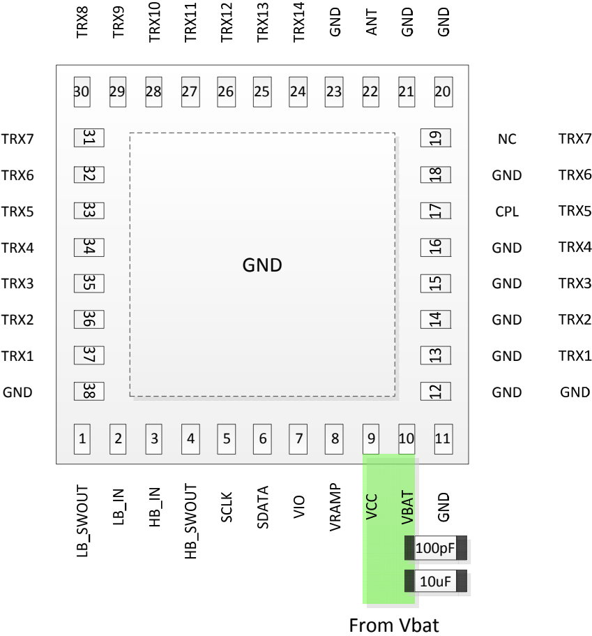
DC Supply
