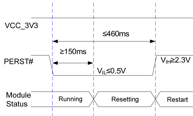
Figure 11: Timing of Resetting Module
