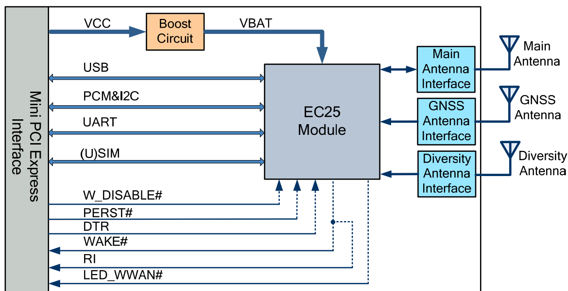
Figure 1: Functional Diagram
