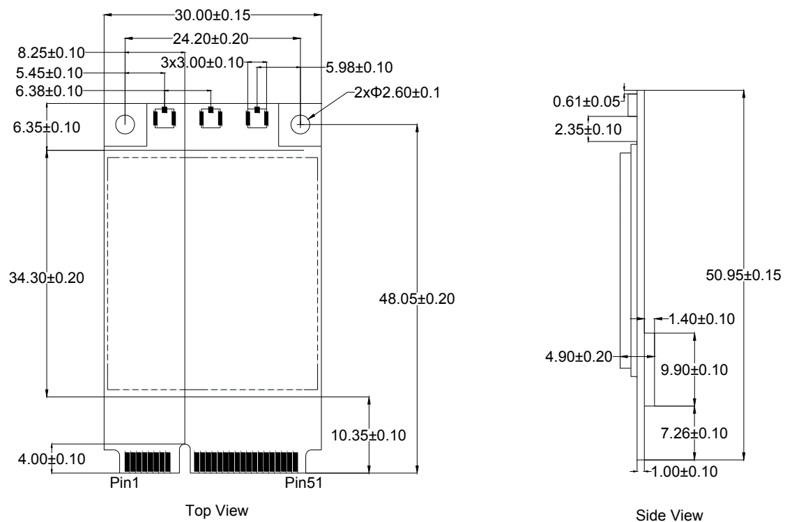
Figure 18: Mechanical Dimensions of EC25 Mini PCIe
