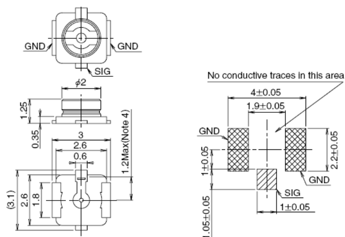
Figure 14: Dimensions of the Antenna Connectors (Unit: mm)
