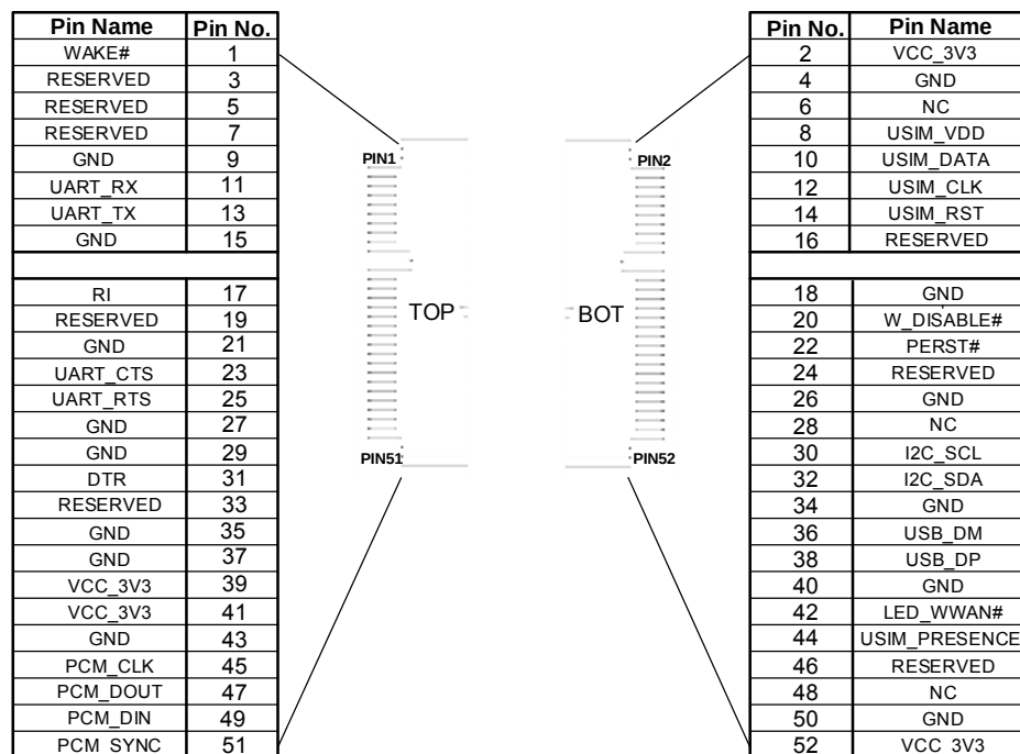
Figure 2: UC200T-GL Mini PCIe Pin Assignment
