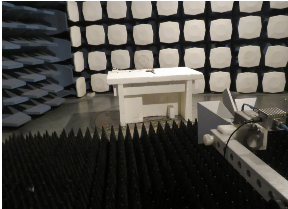
Picture 1: Radiated Spurious Emissions Test setup
