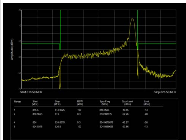
LTE Band 26 16QAM 5MHz CH-High 100%RB
