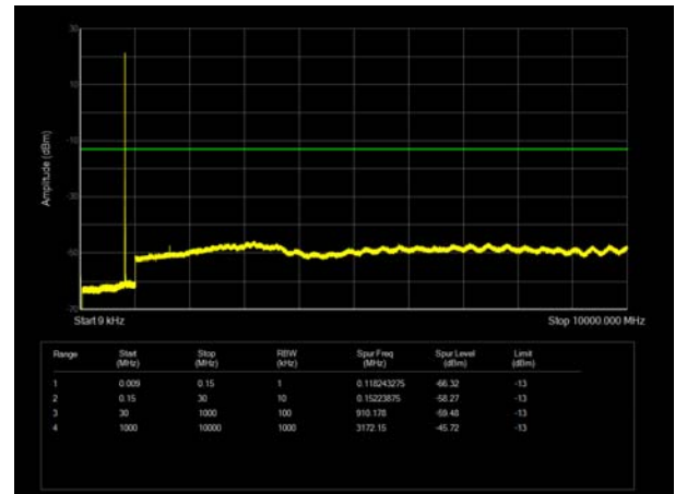
LTE Band 26 3MHz CH Low 9kHz~10GHz
