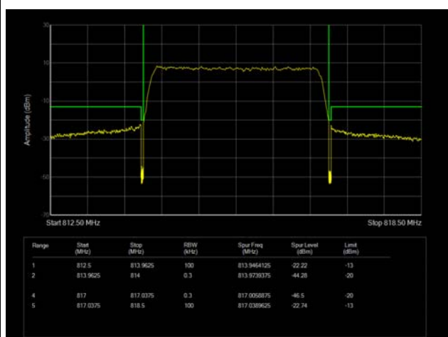
LTE Band 26 16QAM 3MHz CH-Low 100%RB
