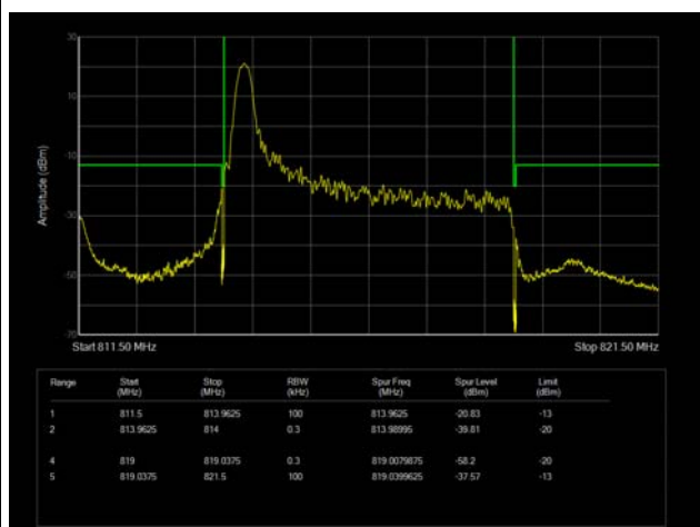
LTE Band 26 16QAM 5MHz CH-Low 100%RB
