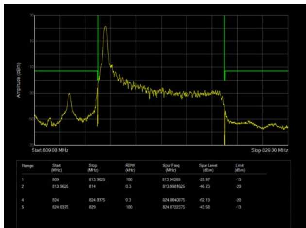
LTE Band 26 QPSK 10MHz CH-Low 100%RB
