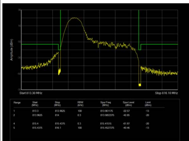
LTE Band 26 16QAM 1.4MHz CH-Low 1RB
