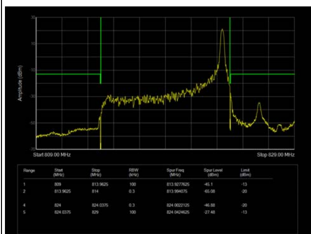
LTE Band 26 16QAM 10MHz CH-High 1RB
