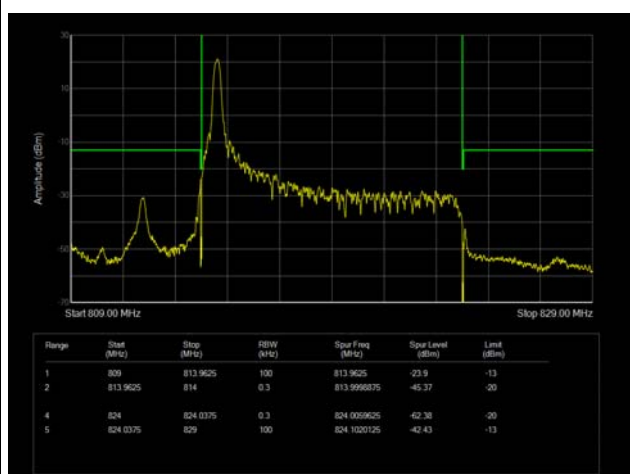
LTE Band 26 16QAM 10MHz CH-Low 1RB
