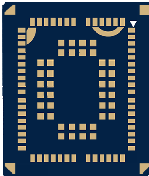
Figure 46: QM95-E Bottom View of the Module
