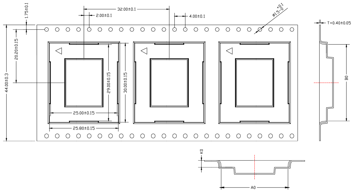
Figure 49: Tape Specifications
