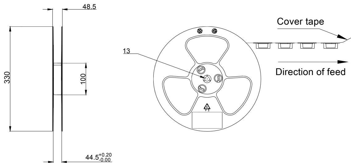
Figure 50: Reel Specifications
