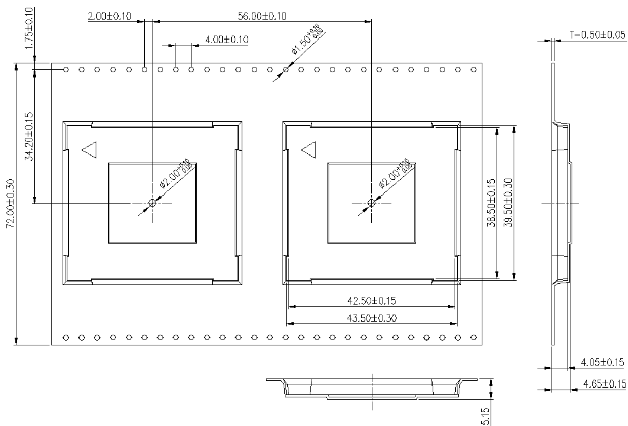
Figure 45: Tape Specifications
