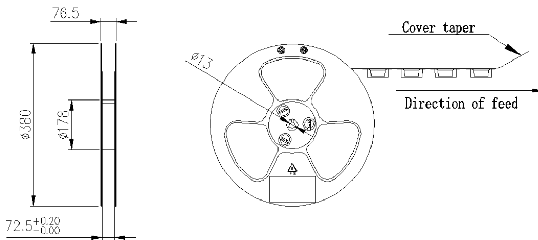
Figure 46: Reel Specifications
