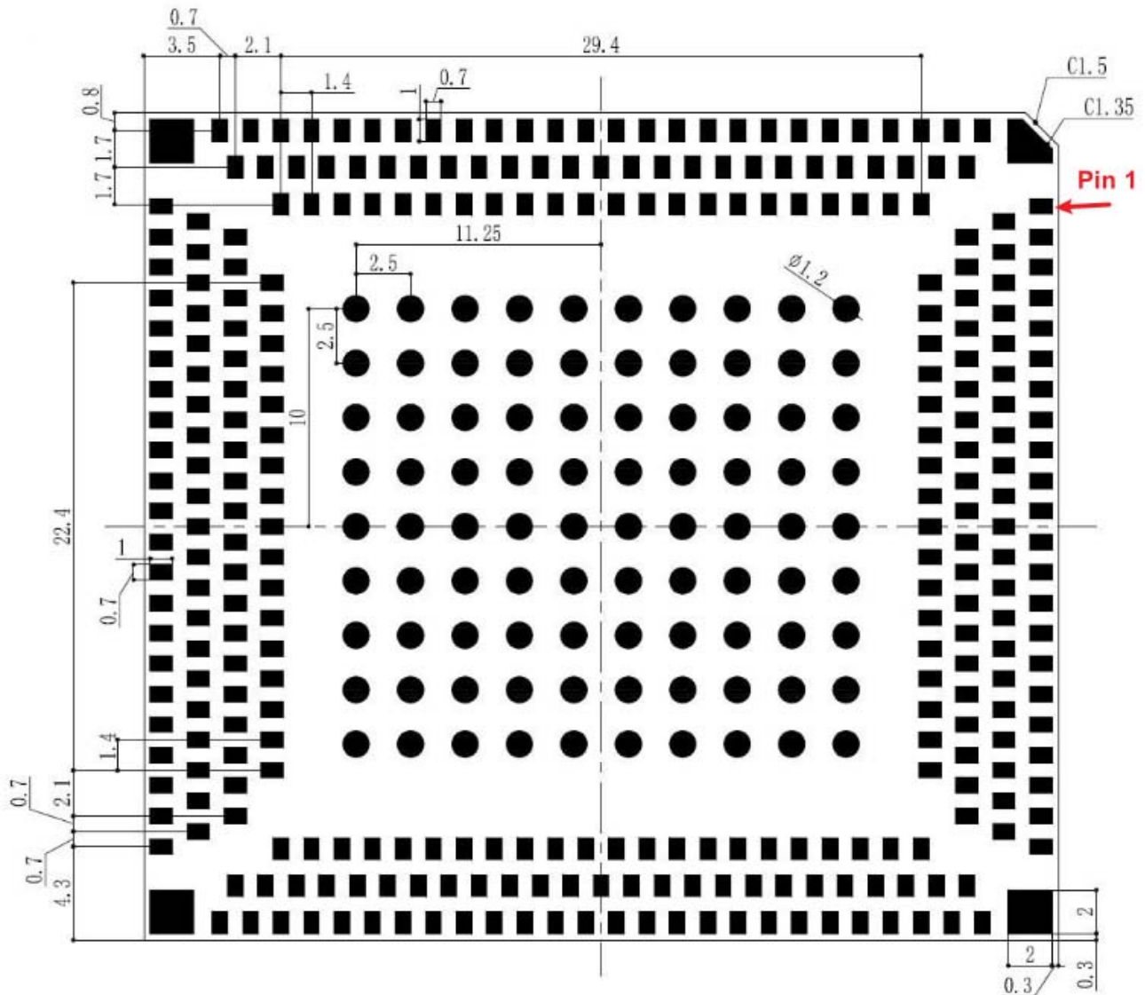
Figure 41: Recommended Footprint (Top View)
