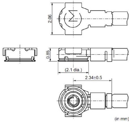
Figure 35: Specifications of Mating Plugs Using Ø0.81 mm Coaxial Cables
