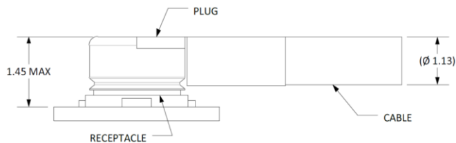
Figure 37: Connection between RF Connector and Mating Plug Using Ø1.13 mm Coaxial Cable
