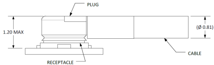
Figure 36: Connection between RF Connector and Mating Plug Using Ø0.81 mm Coaxial Cable
