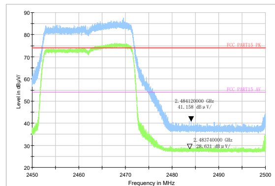
802.11ax HE20 -Channel 11 Peak &amp; Average
