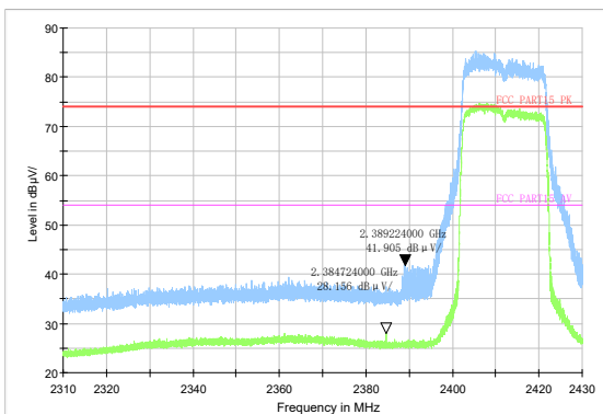
802.11ax HE20 -Channel 1 Peak &amp; Average
