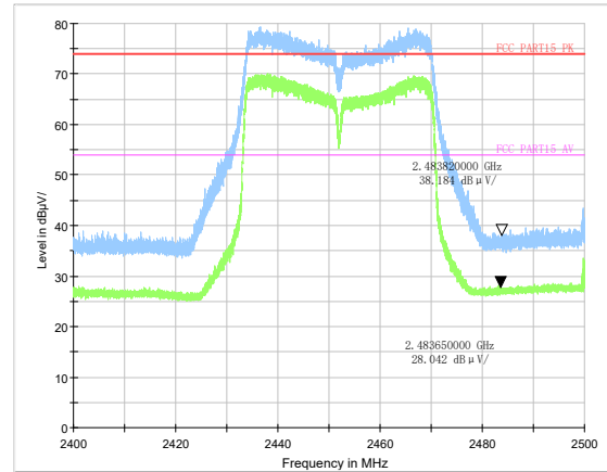
802.11n HT40 -Channel 9 Peak &amp; Average
