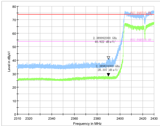
802.11n HT40 -Channel 3 Peak &amp; Average
