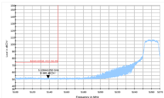
802.11a-Channel 52: Average
