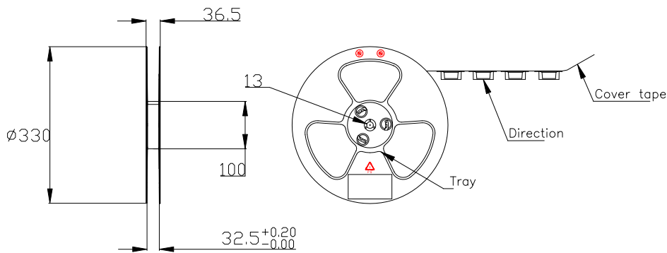
Figure 28: Reel Dimensions
