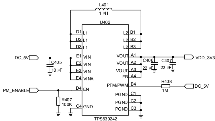
Figure 3: Reference Circuit for VDD_3V3
