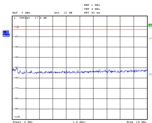
LTE Band 4 1.4MHz CH-Low 3GHz~18GHz
