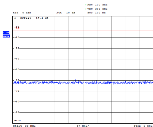
LTE Band 4 1.4MHz CH-Low 30MHz~1GHz
