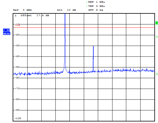
LTE Band 4 1.4MHz CH-Middle 1GHz~3GHz
