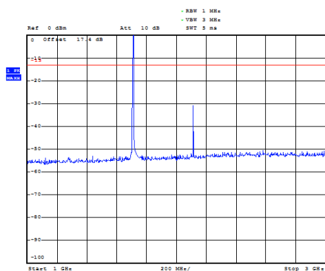
LTE Band 4 1.4MHz CH-Low 1GHz~3GHz
