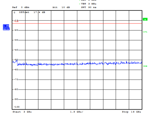
LTE Band 4 1.4MHz CH-Middle 3GHz~18GHz
