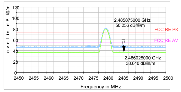
Bluetooth LE Channel 39 Peak+ Average
