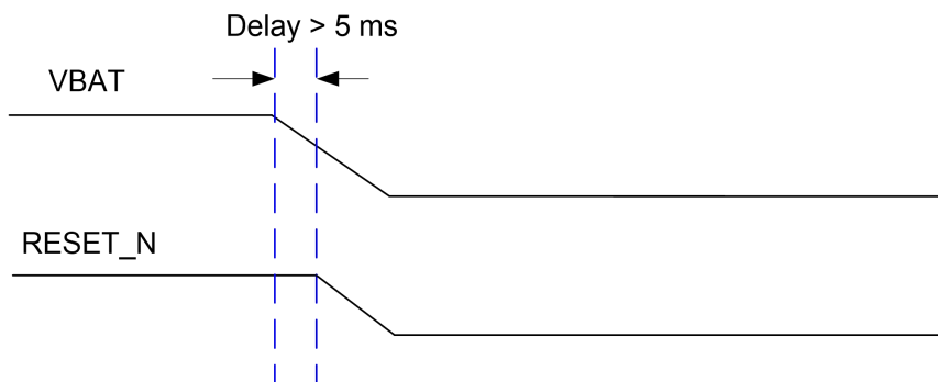
Figure 7: Power-down Timing
