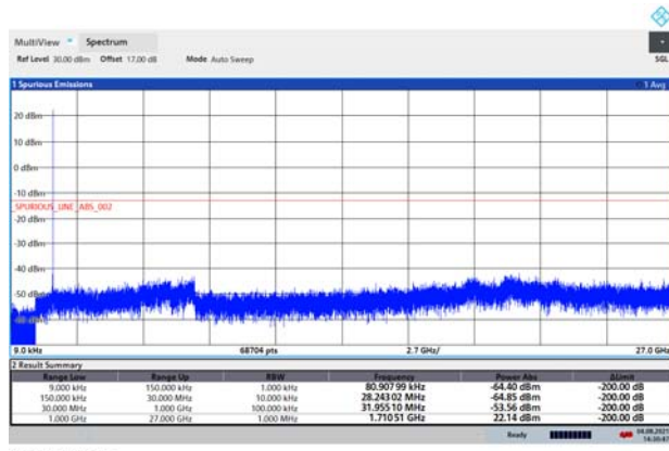
NB-IoT Band 4 CH-Middle 9kHz~27GHz
