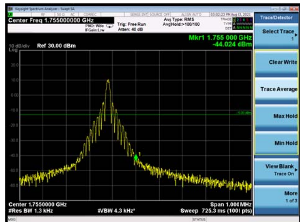
NB-IoT Band 4 BPSK 15KHz 1@0 CH- High
