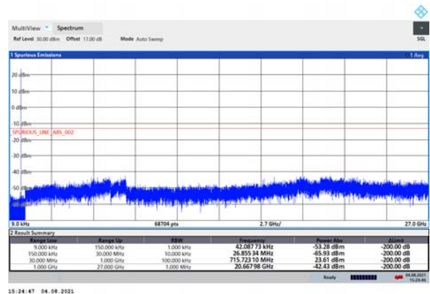
NB-IoT Band 12 CH-High 9kHz~27GHz
