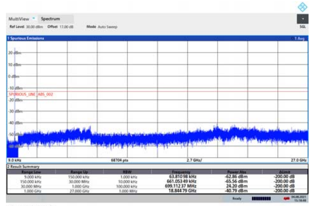
NB-IoT Band 12 CH-Middle 9kHz~27GHz
