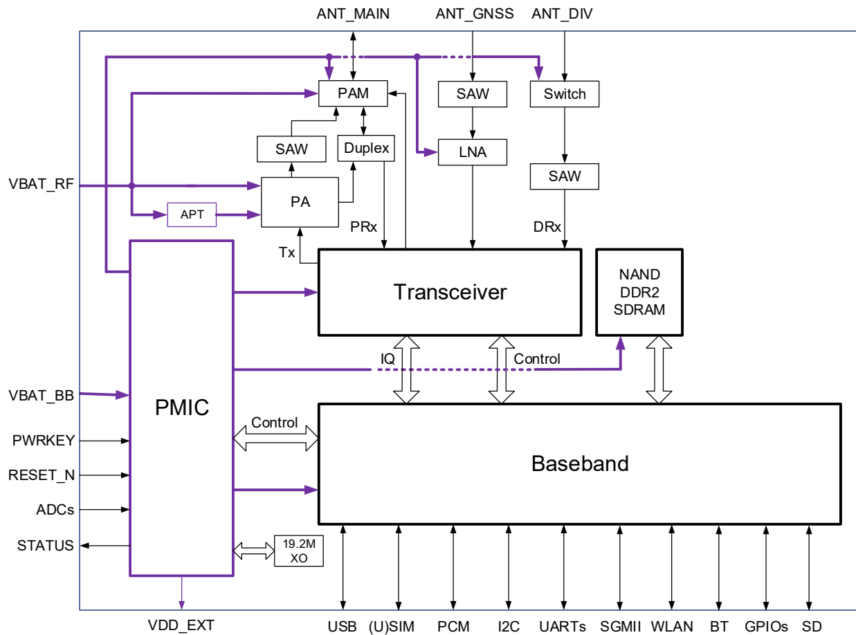
Figure 1: Functional Diagram
