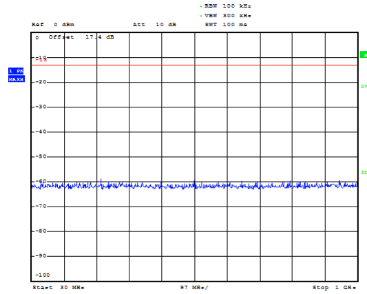
LTE Band 2 1.4MHz CH-Middle 30MHz~1GHz
