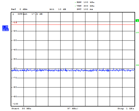
LTE Band 2 1.4MHz CH-Low 30MHz~1GHz
