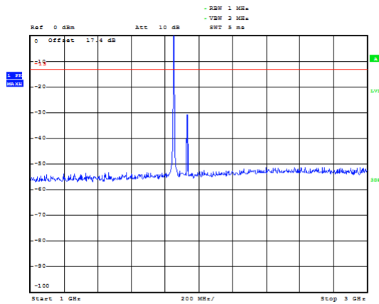
LTE Band 2 1.4MHz CH-Low 1GHz~3GHz
