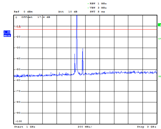
LTE Band 2 1.4MHz CH-Middle 1GHz~3GHz
