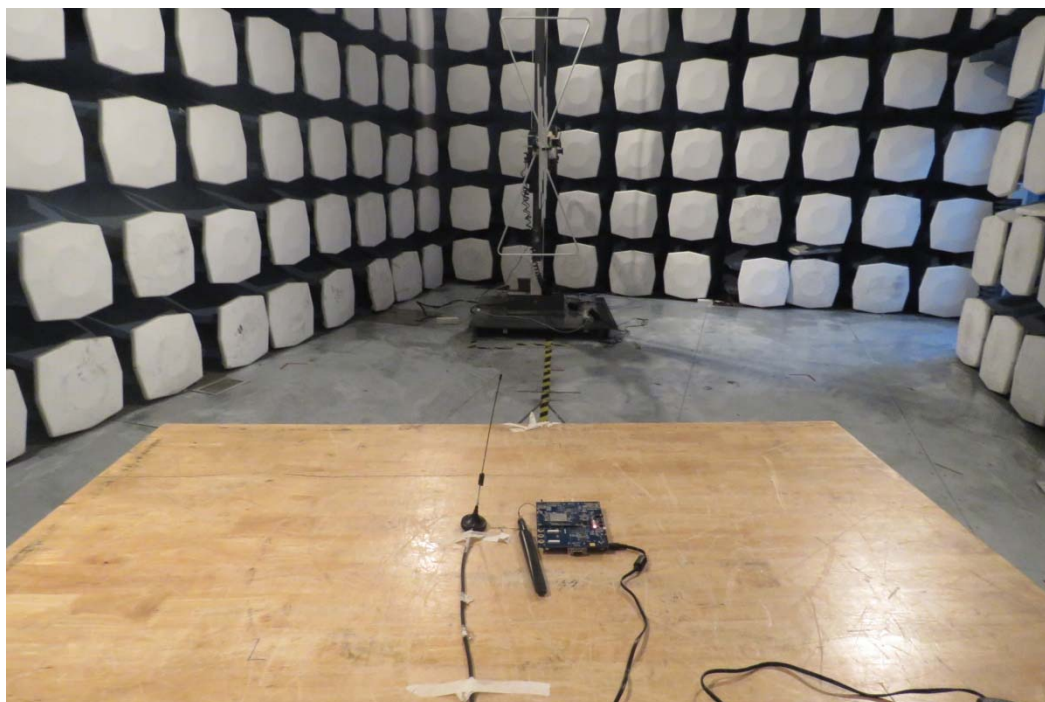
30MHz-1GHz
