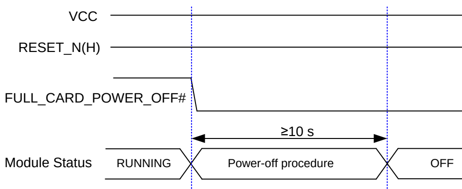
Figure 10: Turn-off Timing through FULL_CARD_POWER_OFF#
