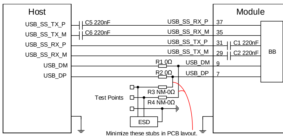
Figure 20: Reference Circuit of USB 3.1 & 2.0 Interface
