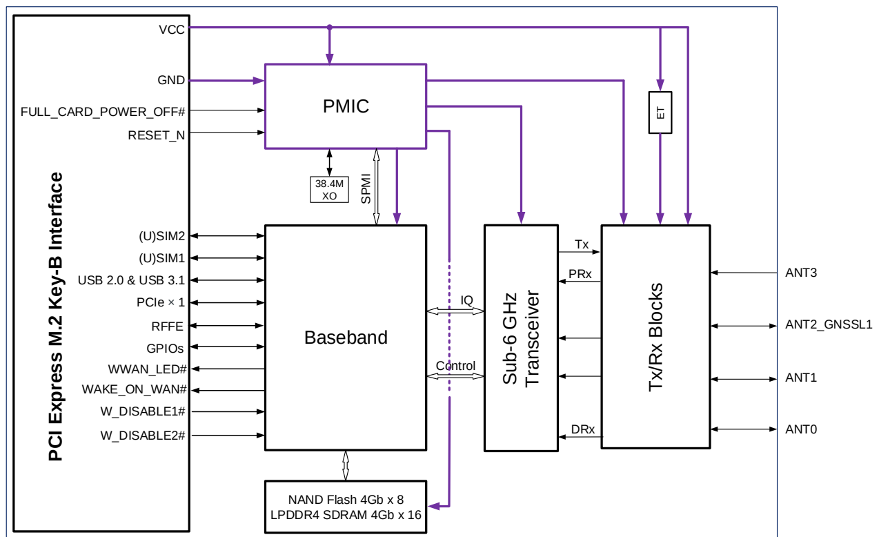
Figure 1: Functional Diagram
