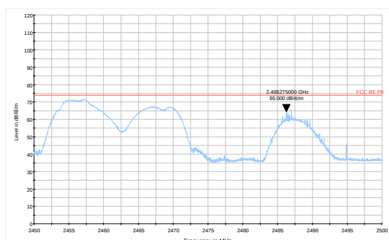
802.11g-Channel 11 Peak
