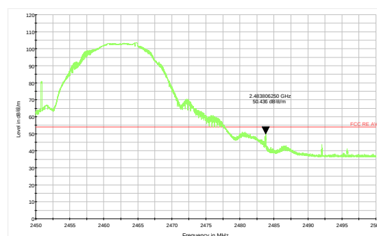
802.11b-Channel 11 Average
