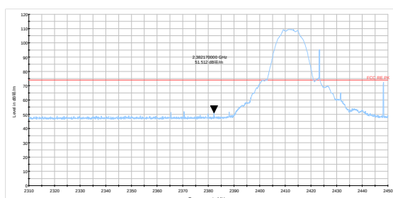
802.11b-Channel 1 Peak
