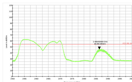
802.11g-Channel 11 Average
