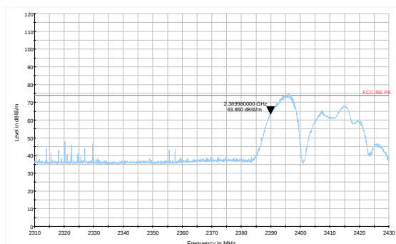
802.11g-Channel 1 Peak
