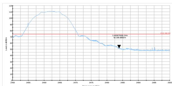
802.11b-Channel 11 Peak
