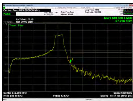
LTE Band 5 QPSK 1.4MHz CH-High 100%RB
