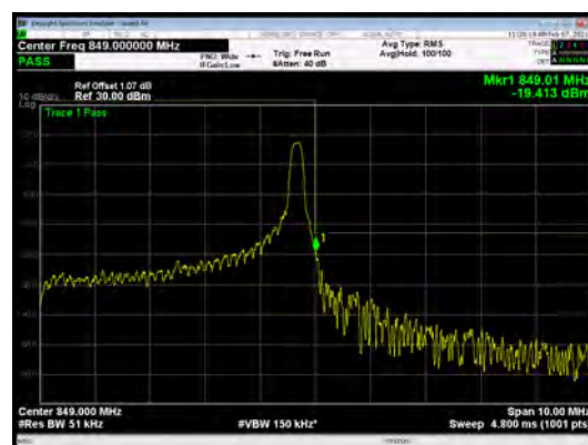
LTE Band 5 16QAM 5MHz CH-High 100%RB
