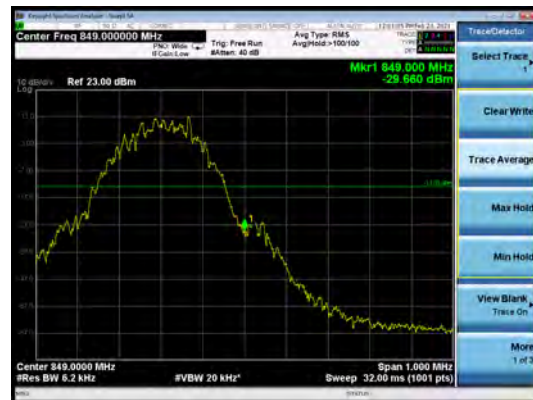
GSM 850 GPRS CH-High
