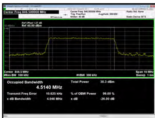
LTE Band 5 16QAM 5MHz CH-High
