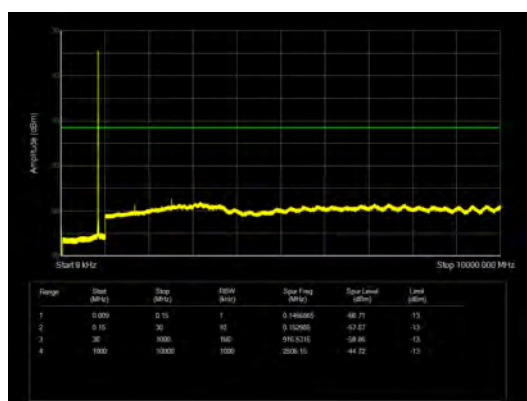
LTE Band 5 3MHz CH-High 9kHz~10GHz
