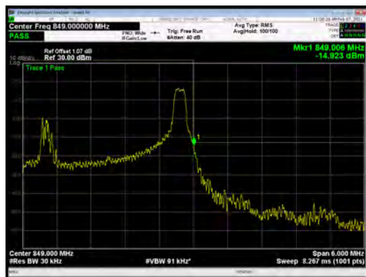
LTE Band 5 QPSK 3MHz CH-High 1RB
