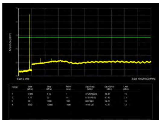
LTE Band 5 3MHz CH-Middle 9kHz~10GHz
