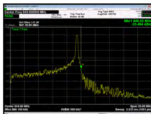
LTE Band 5 16QAM 10MHz CH-High 1RB
