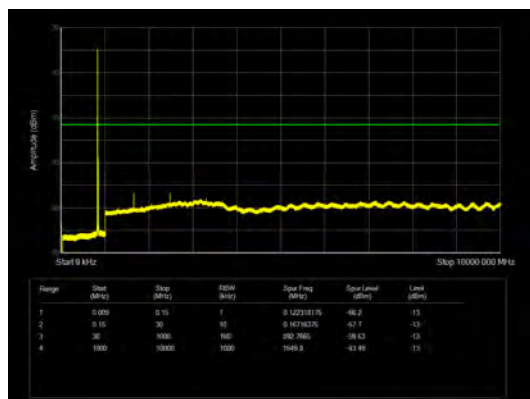
LTE Band 5 10MHz CH-Middle 9kHz~10GHz
