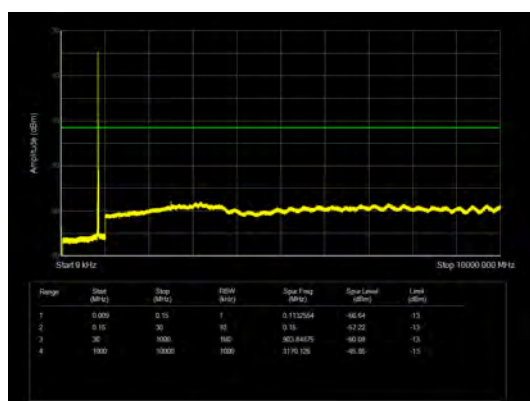
LTE Band 5 10MHz CH-High 9kHz~10GHz
