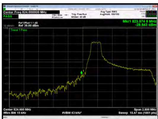
LTE Band 5 16QAM 1.4MHz CH-Low 100%RB
