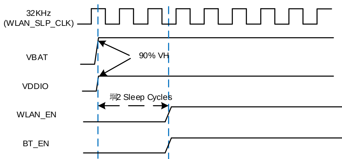
Figure 3: Turn Up Timing
