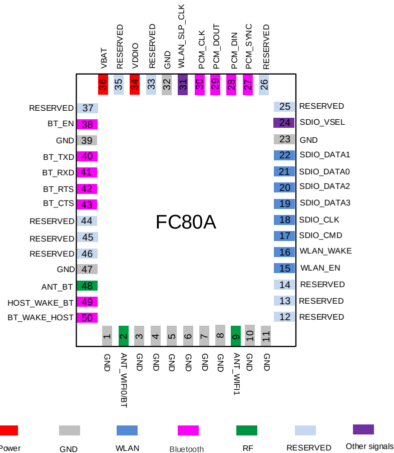
Figure 2: Pin Assignment (Top View)
