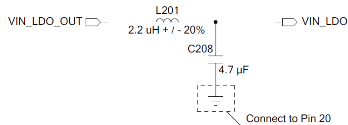
Figure 4: Recommended Reference Design Circuit
