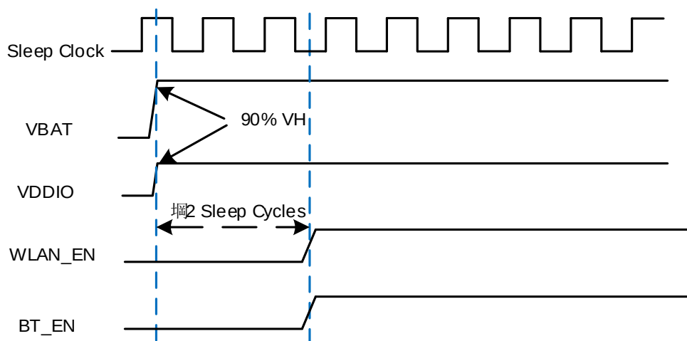
Figure 3: Power-up Timing
