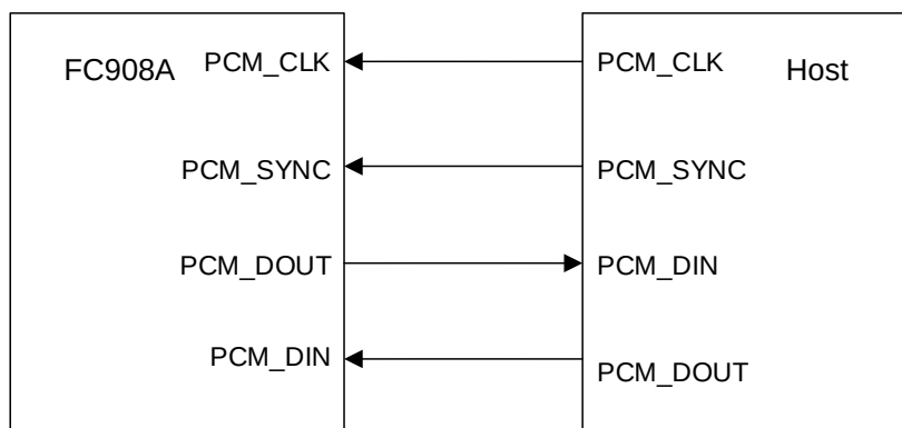
Figure 9: PCM Interface Connection
