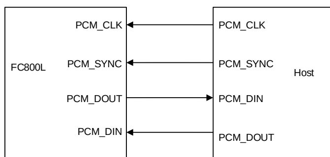
Figure 7: PCM Interface Connection
