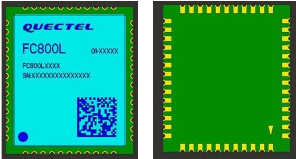
Figure 18: Top and Bottom Views of the Module
