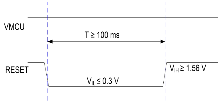
Figure 6: Reset Timing
