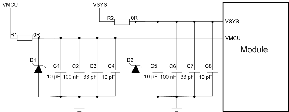
Figure 3: Reference Circuit of Power Supply
