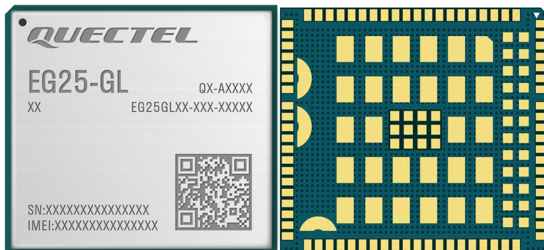
Figure 46: Top and Bottom Views of the Module
