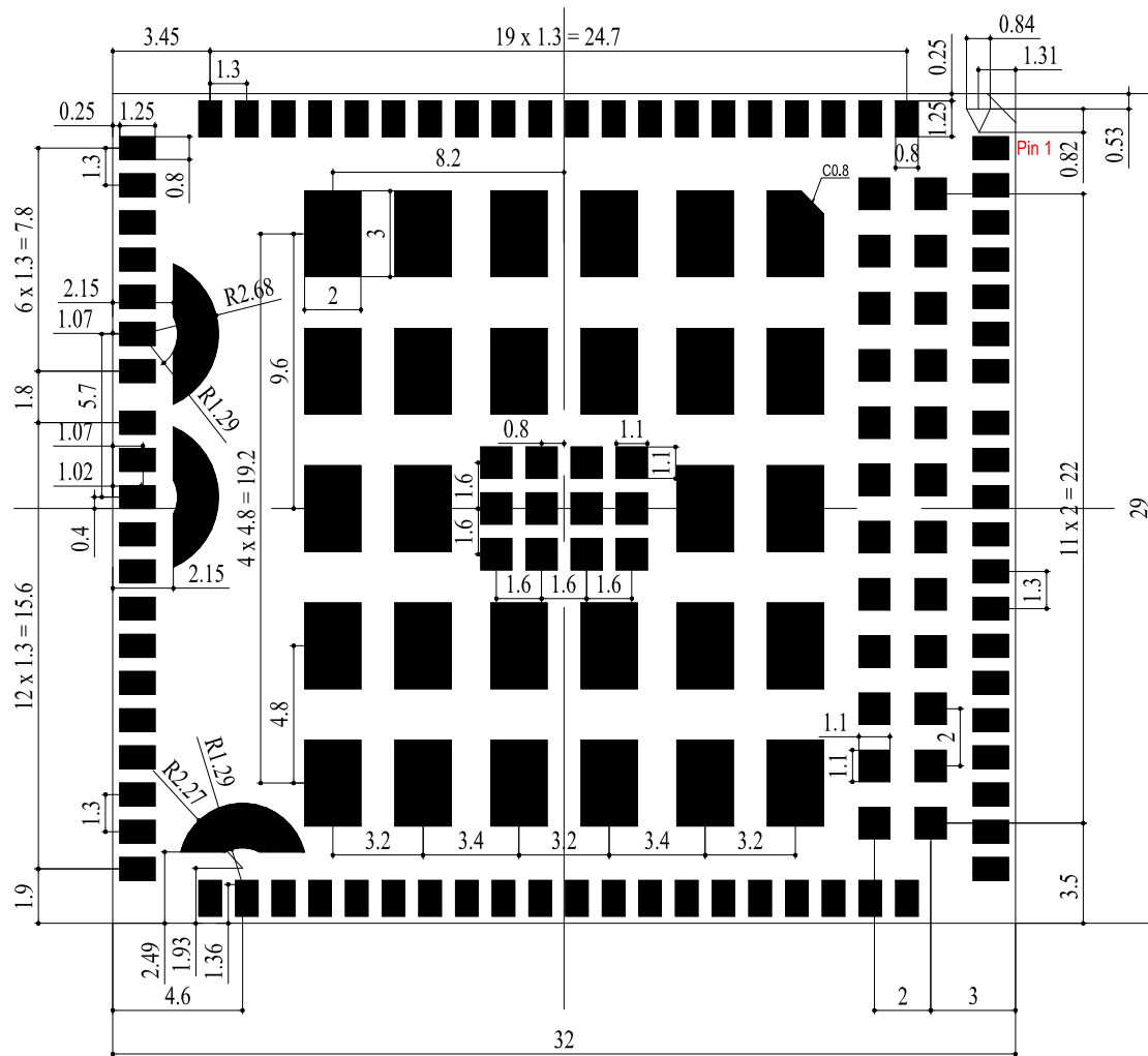
Figure 43: Bottom Dimensions (Bottom View)
