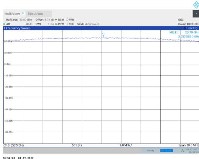
Band48-5MHz-QPSK-55265-1RB#12
