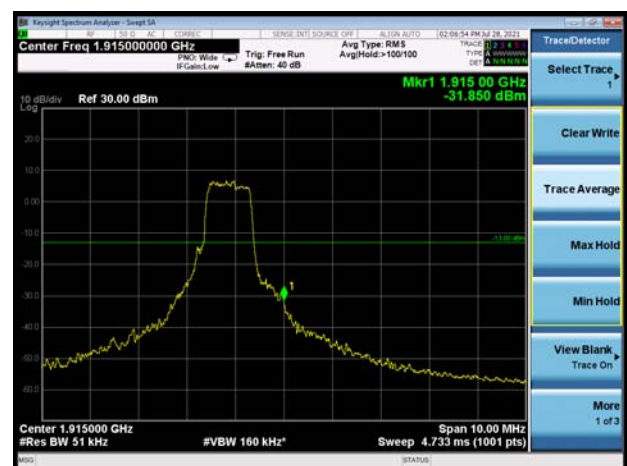
LTE Band 25 10MHz 16QAM 100%RB CH-High
