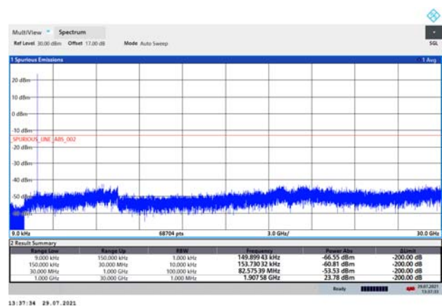
LTE Band 2 3MHz CH-High 9kHz~30GHz
