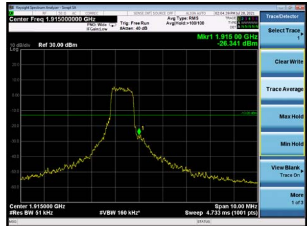
LTE Band 25 10MHz 16QAM 1RB CH-High
