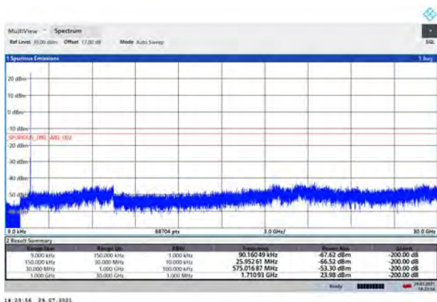
LTE Band 4 3MHz CH-Middle 9kHz~30GHz
