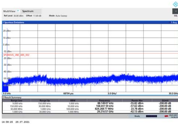
LTE Band 5 1.4MHz CH-Middle 9kHz~30GHz
