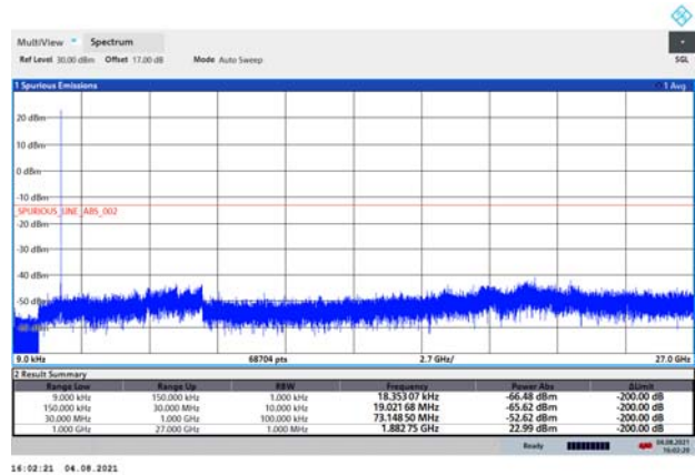
NB-IoT Band 25 CH-High 9kHz~27GHz
