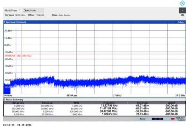
NB-IoT Band 25 CH-Middle 9kHz~27GHz
