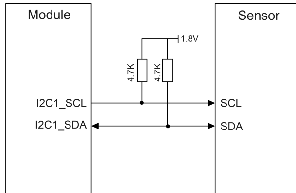
Figure 19: Reference Design of I2C Interface with an External I2C Interface Sensor
