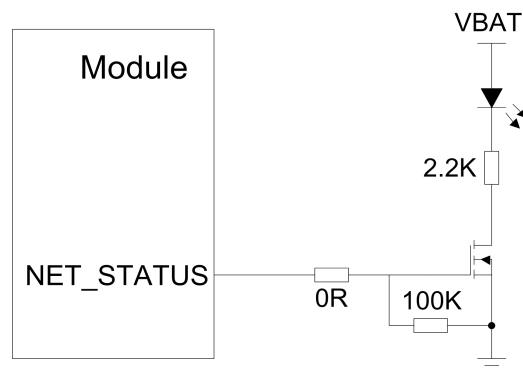
Figure 20: Reference Design of NET_STATUS
