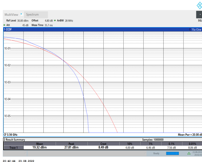
Band48-20MHz-QPSK-55990-100RB#0
