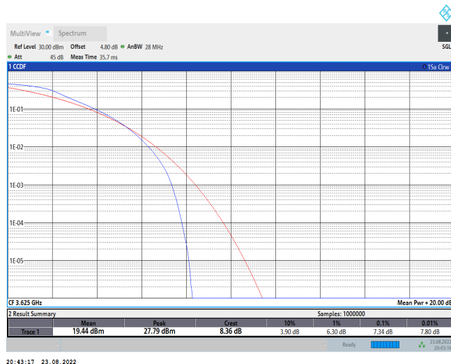
Band48-20MHz-QPSK-55990-100RB#0
