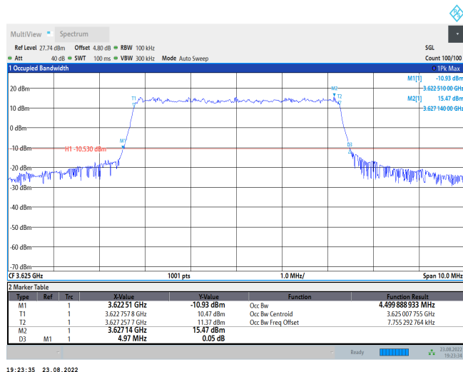
Band48-5MHz-QPSK-55990-25RB#0
