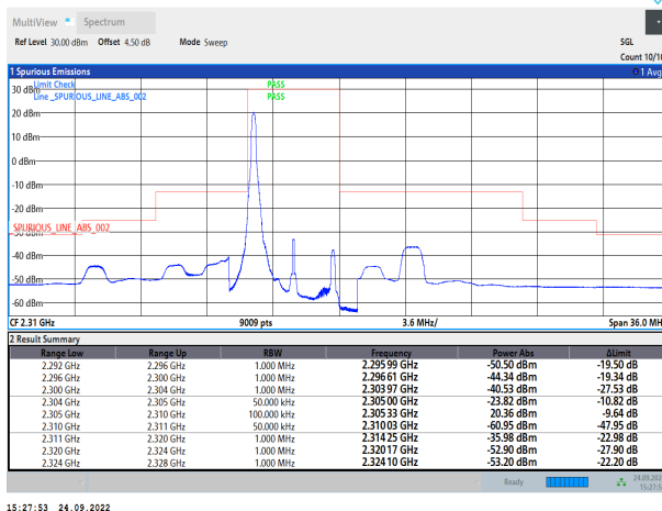
Band30-5MHz-QPSK-27685-25RB#0
