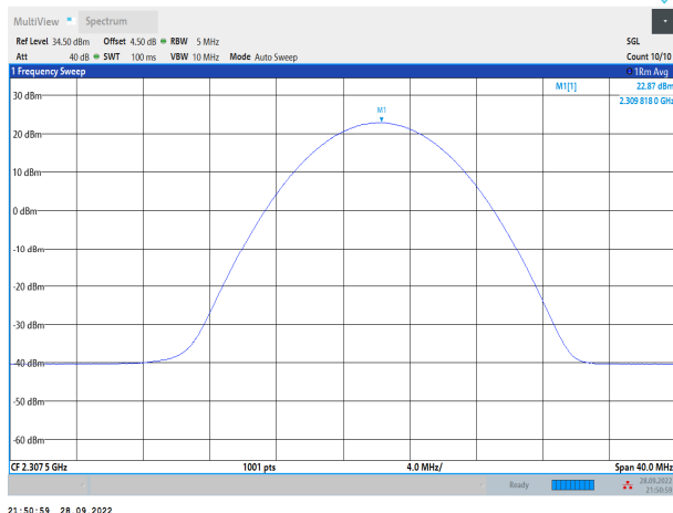
Band30-5MHz-QPSK-27685-1RB#24
