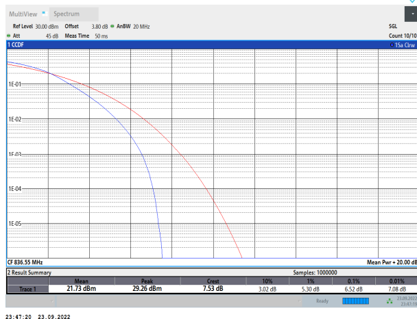
5-5-10MHz-10MHz-QPSK-QPSK-20476-20575-50RB#0-50RB#0
