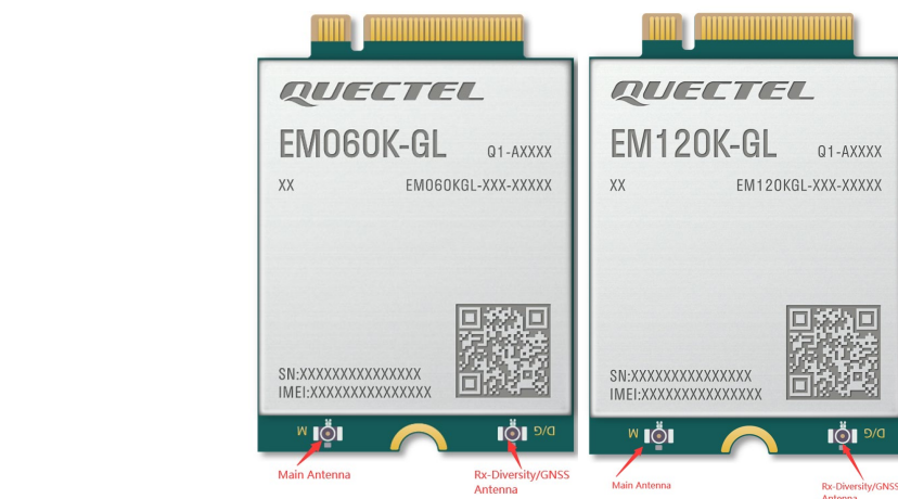
Figure 26: Antenna Connectors on the EM060K-GL and EM120K-GL
