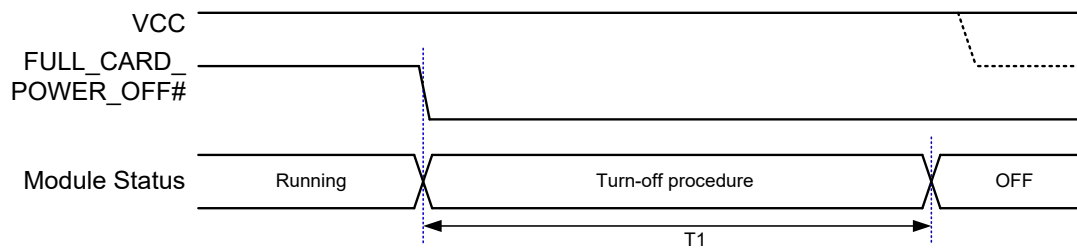
Figure 10: Turn-off Timing through FULL_CARD_POWER_OFF#
