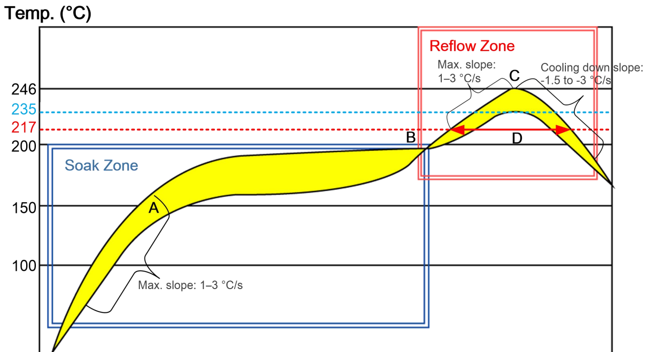
Figure 25: Recommended Reflow Soldering Thermal Profile
