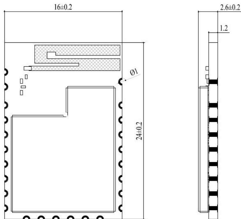
Figure 19: Module Top and Side Dimensions for FCM100D_PCB_Antenna
