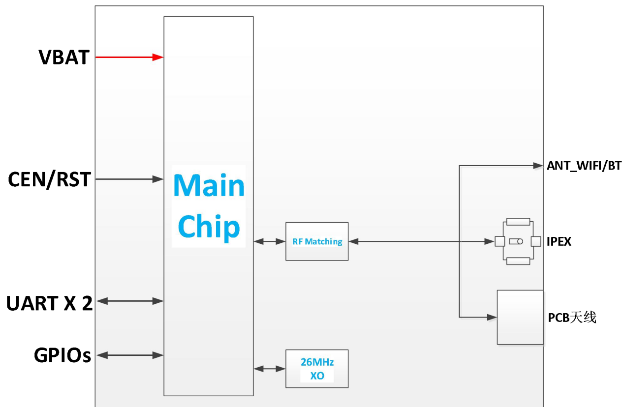
Figure 1: Functional Diagram
