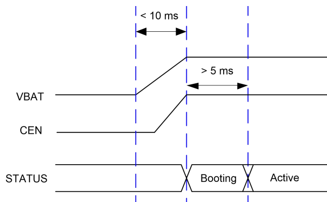
Figure 4: Power-up Timing
