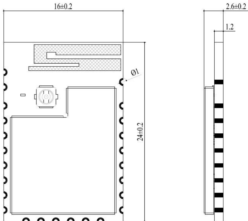
Figure 20: Module Top and Side Dimensions for FCM100D_IPEX
