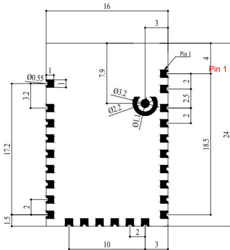
Figure 22: Module Dimension (Bottom View)
