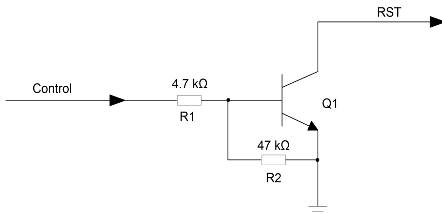
Figure 5: Reference Circuit of CEN by Using Driving Circuit
