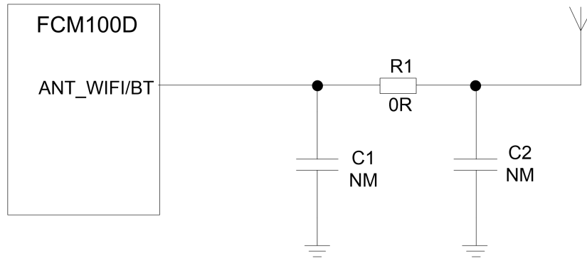
Figure 10: RF Antenna Reference Design
