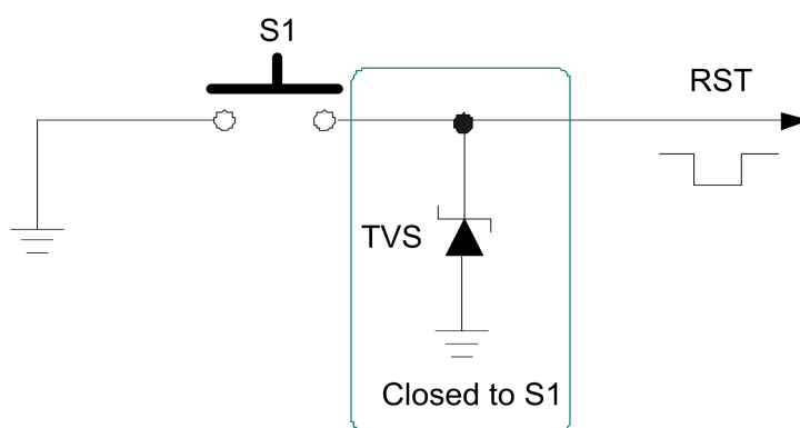
Figure 6: Reference Circuit of CEN by Using Button
