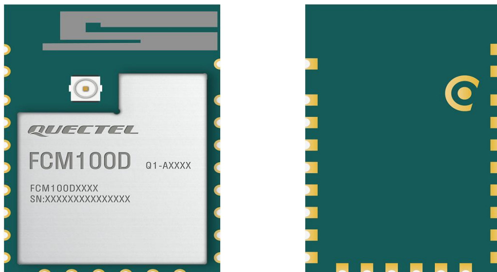
Figure 24: Top and Bottom Views of the Module
