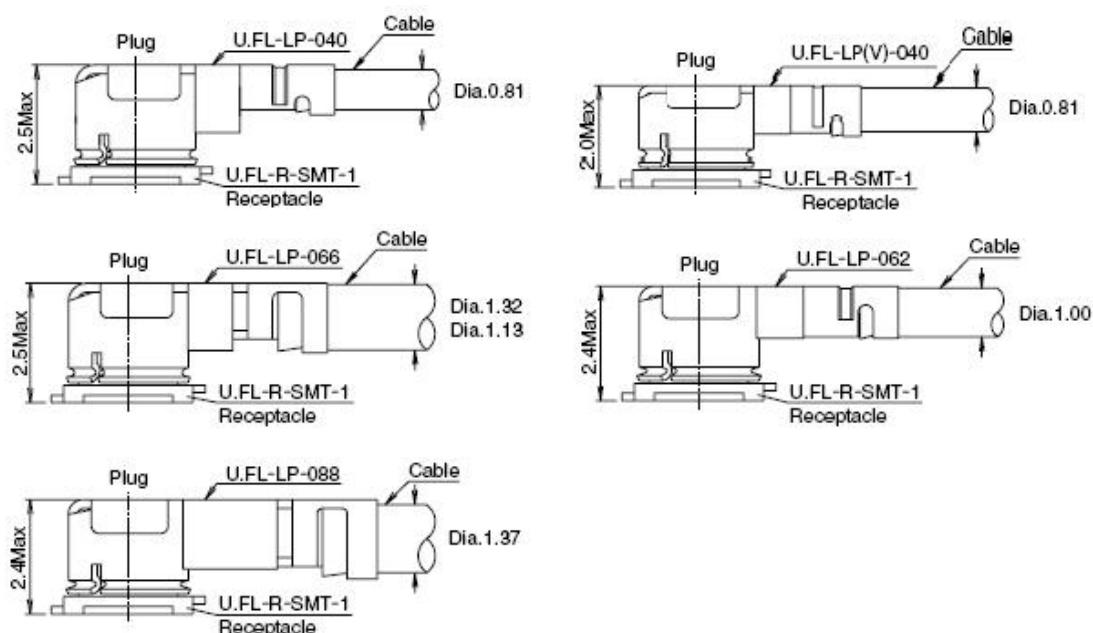
Figure 18: RF Connectors assembling
