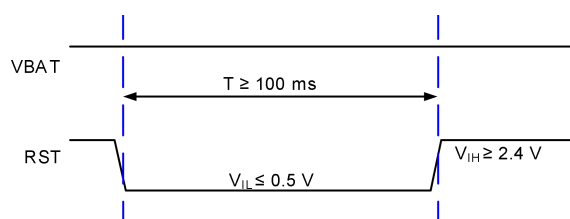
Figure 7: Timing of Resetting the Module
