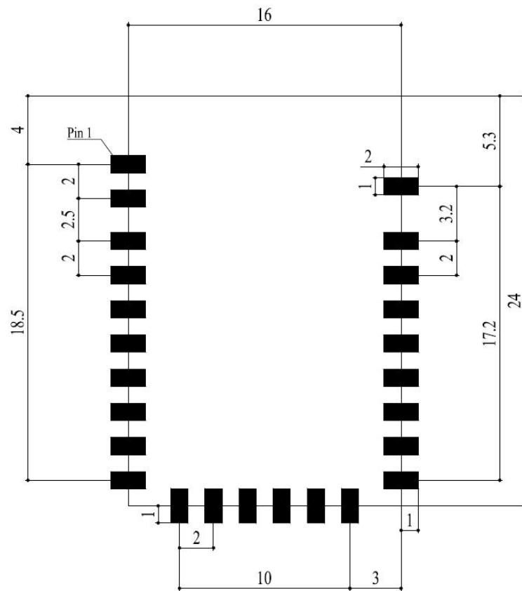
Figure 23: Recommended Footprint (Top View)
