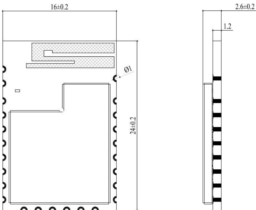
Figure 21: Module Top and Side Dimensions for FCM100D_LCC
