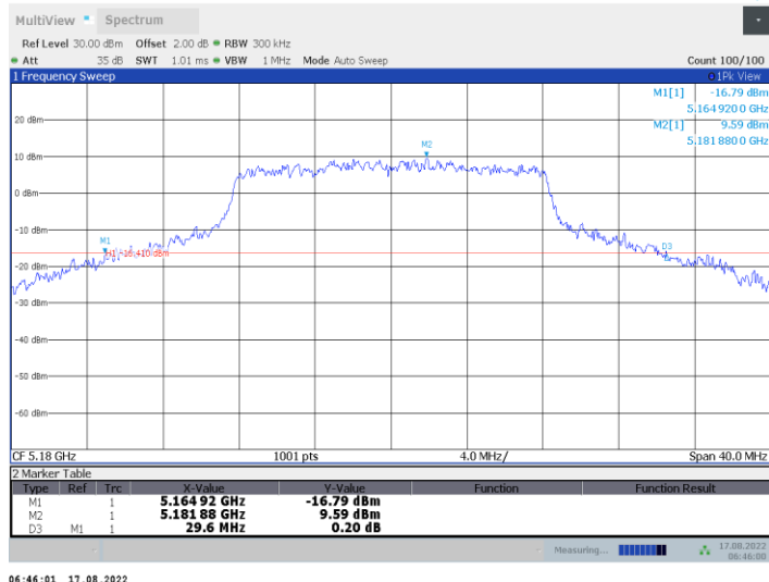
11a-CDD Ant2 5180
