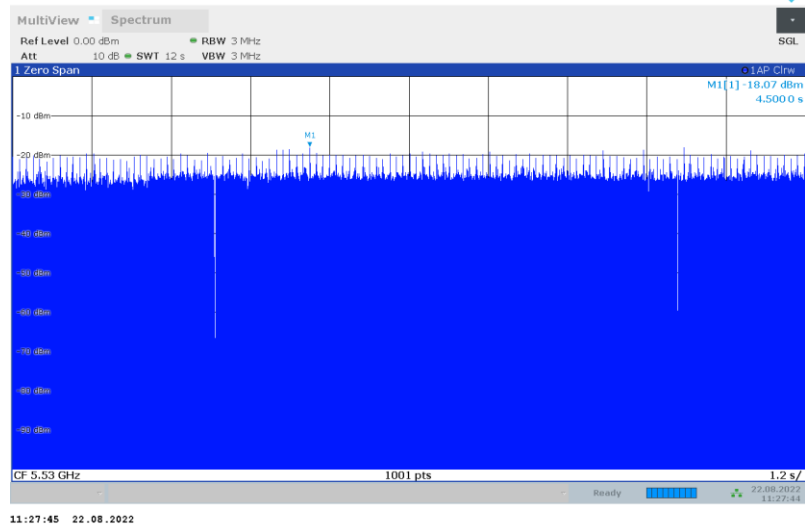
Master—11ac80MIMO_5530
