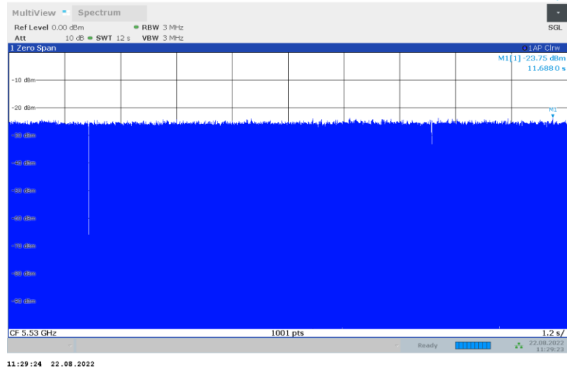
Master—11ac80MIMO_5530
