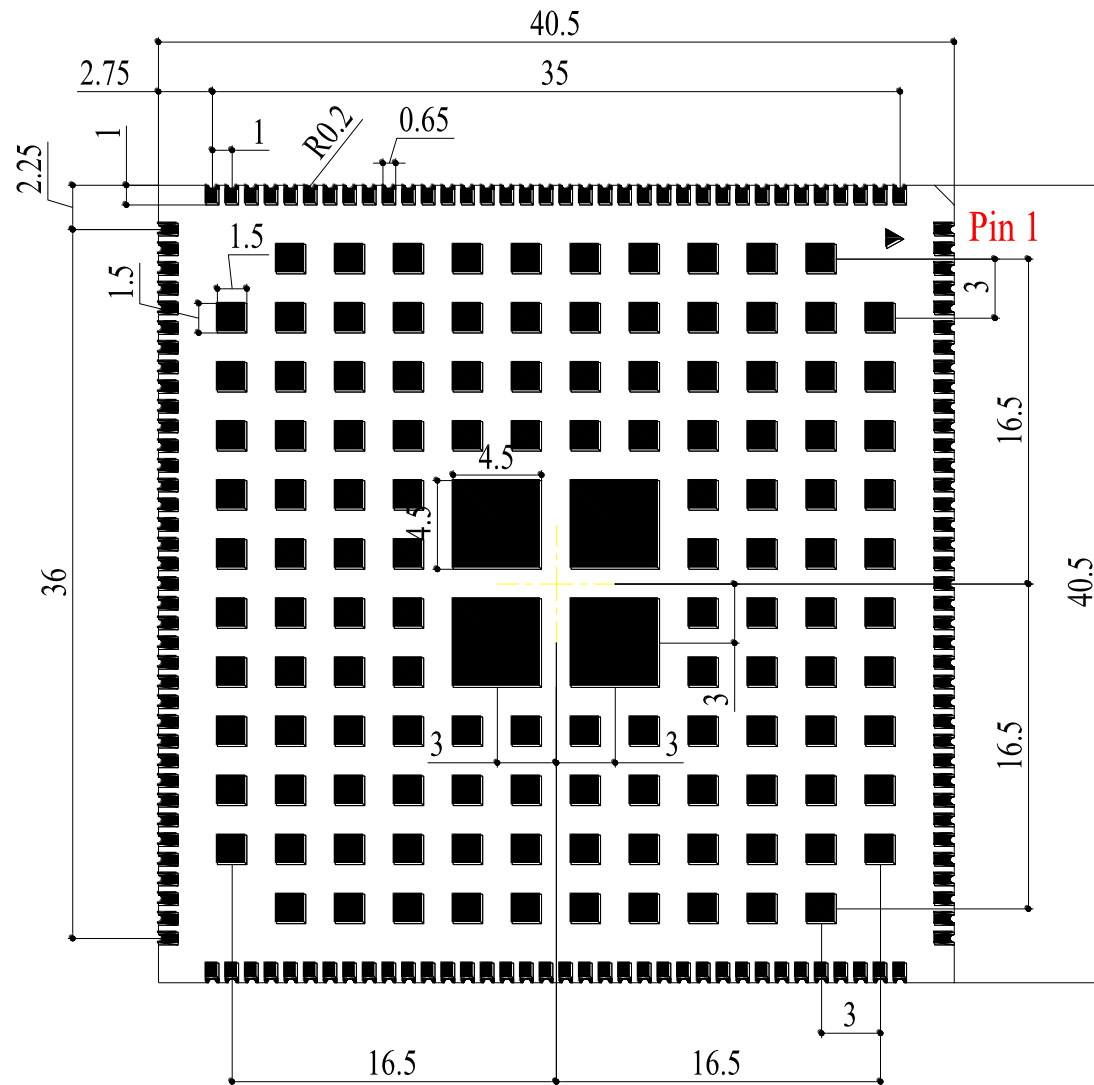
Figure 40: Module Bottom Dimensions (Bottom View)
