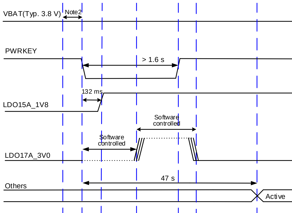
Figure 7: Turn-on Timing
