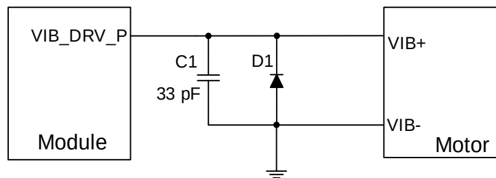
Figure 17: Reference Circuit for Motor Connection
