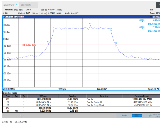
Band26-1.4MHz-QPSK-26740-6RB#0
