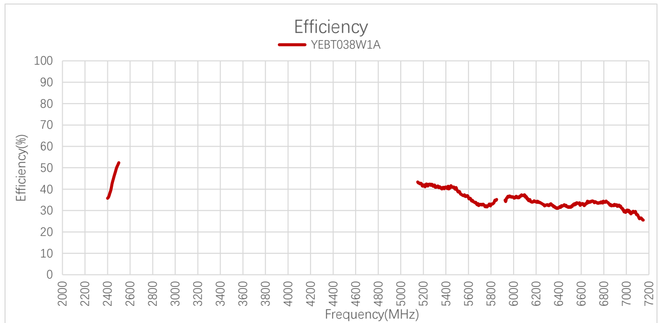
Efficiency (%)
