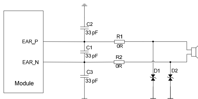
Figure 20: Reference Design of Earpiece Interface
